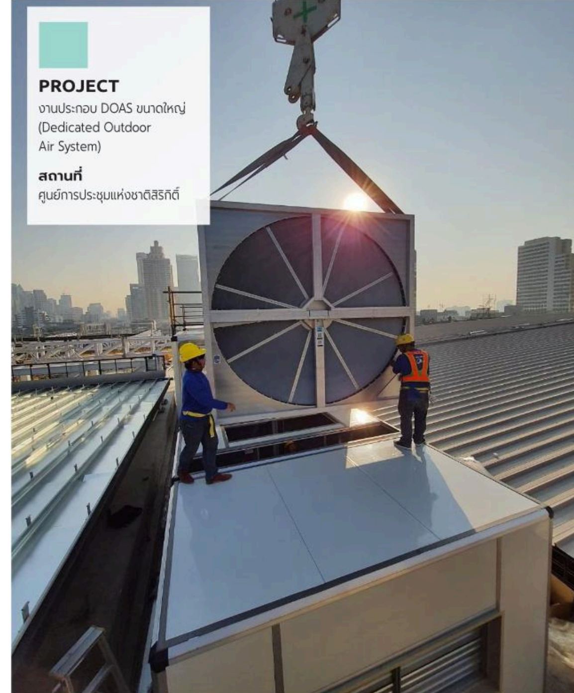
Ventilation System
